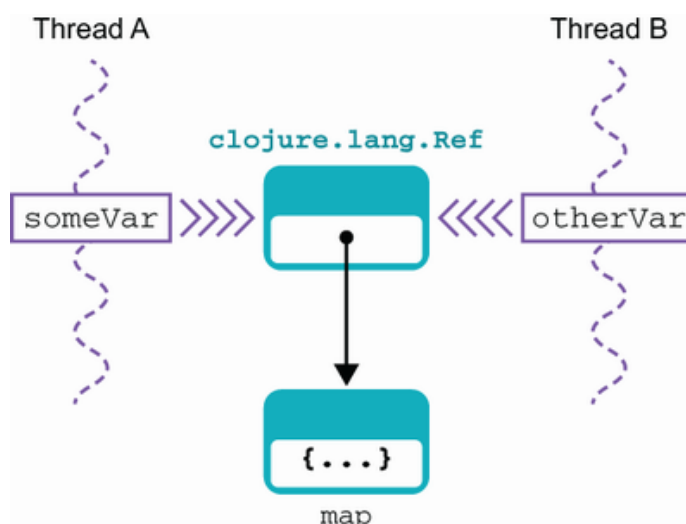
Figure 16.10 Software transactional memory
