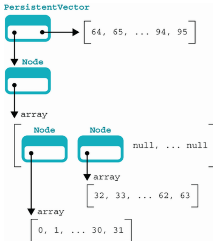
Figure 16.7 A persistent vector with 96 elements
