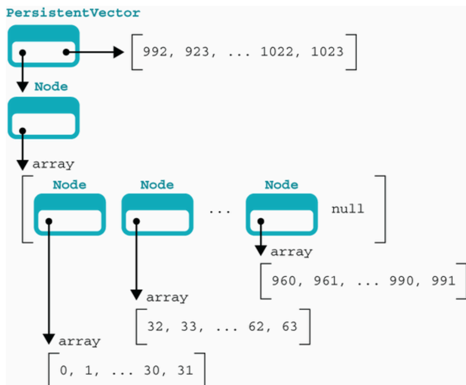
Figure 16.8 A persistent vector with 1,056 elements
