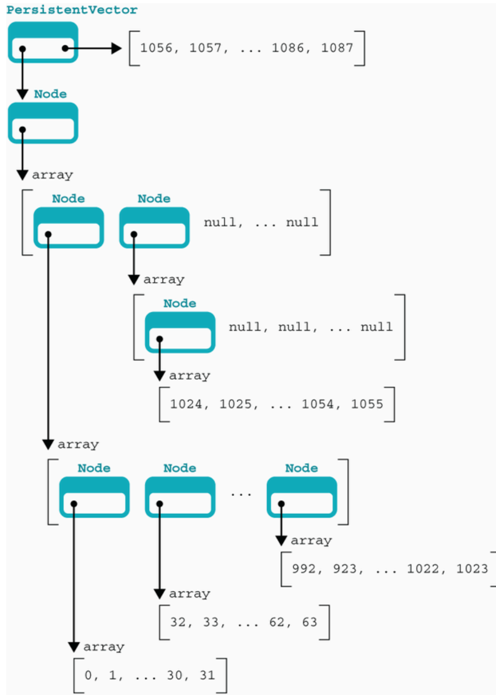
Figure 16.9 A persistent vector with many elements
