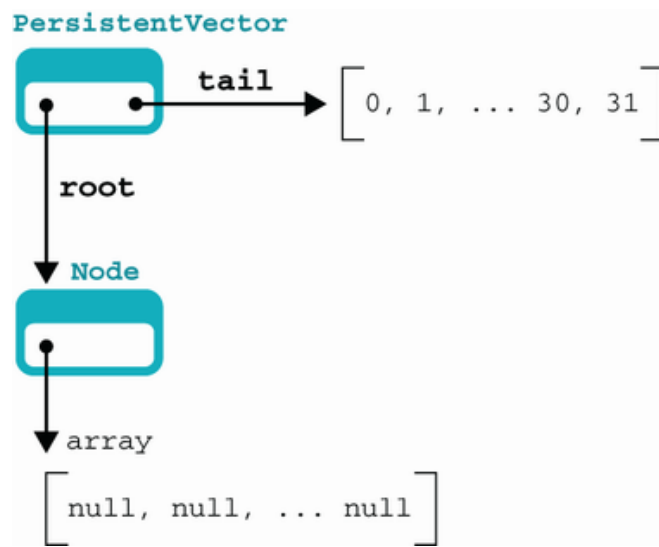
Figure 16.5 A persistent vector with 32 elements
