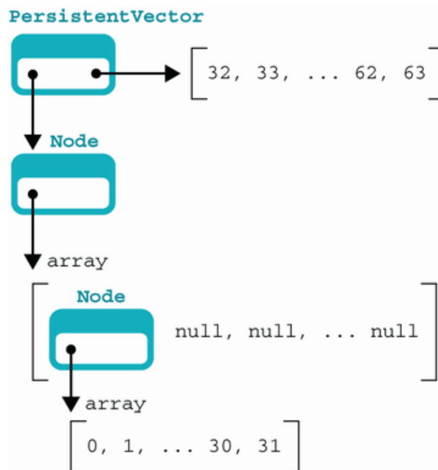
Figure 16.6 A persistent vector with 64 elements
